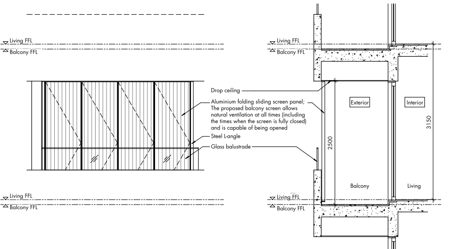
Garden Block Typical Retractable Balcony Screen - Elevation
